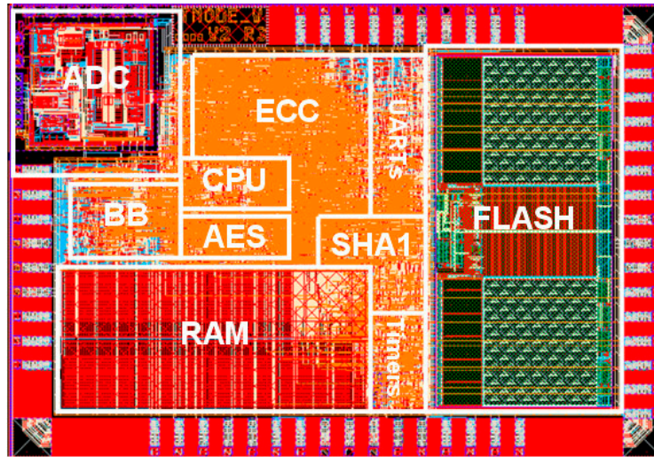
Figure 4. Layout of the TNODE5 chip.
