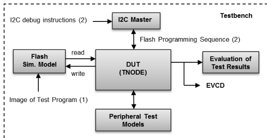
Figure 5. TNODE5 testbench: (1) Test execution from Flash; (2) Test execution via I 2 C debug port.
