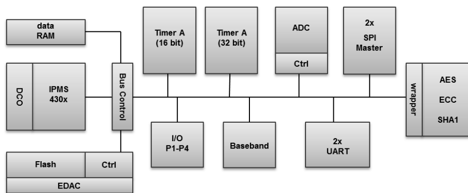
Figure 2. Architecture of TNODE5 microcontroller.
