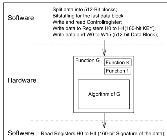
Figure 3. Hash generation flow.
