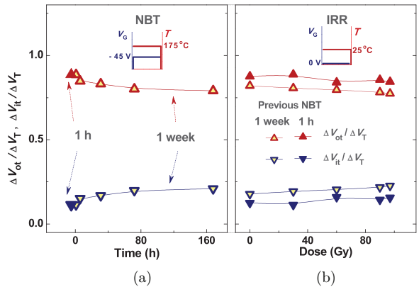
Fig. 10. Contributions of gate oxide charge and interface traps relative to the threshold voltage shift during: (a) static NBT stress and (b) irradiation without gate polarization.
