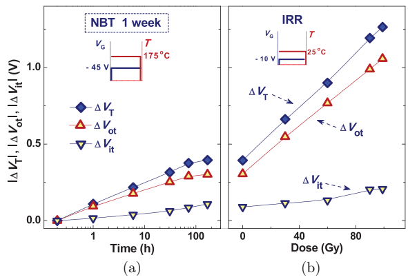
Fig. 7. The threshold voltage shift, contributions of gate oxide charge and interface traps during: (a) static NBT stress and (b) irradiation (with gate polarization), for components NBT stressed during 1 week.
