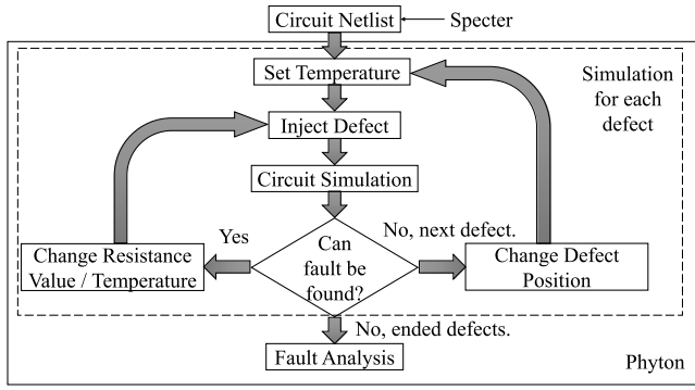
Fig. 6. Simulation flow.
