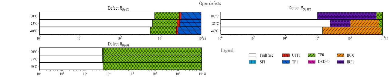
Fig. 9. Open defects: Faults propagated assuming different defect sizes.
