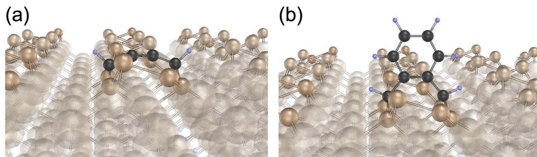
Figure 8. Influence of a dimer vacancy defect on the graphene growth. (a) C 4 H 2 and (b) C 8 H 6 molecules inside a dimer vacancy defect on Ge(001)- p (2 × 2).
