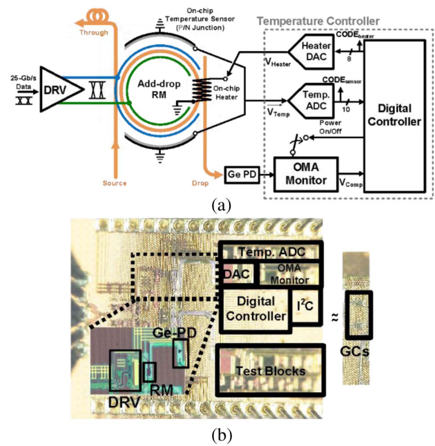
Fig. 3. (a) Block diagram and (b) fabricated chip photo of the monolithic silicon photonic transmitter with a temperature controller.
