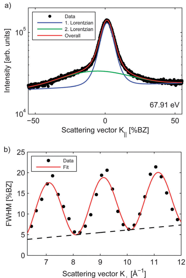
Fig. 3 Spot profile analysis of the Ce 0.65 Pr 0.35 O 2-δ sample after annealing at 400 °C for 30 min. (a) Cross section along the [11 \bar{2} ] direction. The central peak (blue) and the shoulder (green) are fitted with Lorentzian functions. (b) FWHM of the central peak against K_{\perp} . The fit according to eqn (1) is in good agreement with the experimental data.
