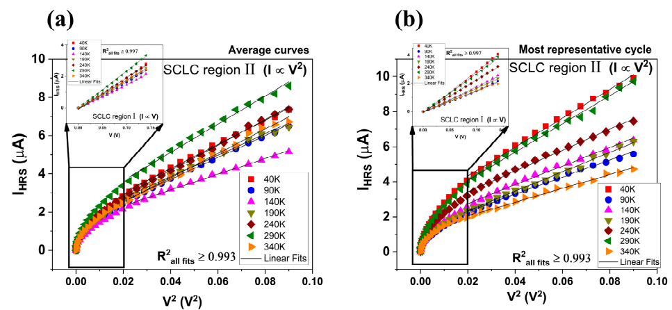
Figure 4. Space-charge-limited conduction plot of I_{\text{HRS}} vs. V^2 at every temperature. Insets: ohmic plot representing region (i) of the SCLC mechanism. (a) Average curves and (b) most representative cycle at each temperature.
