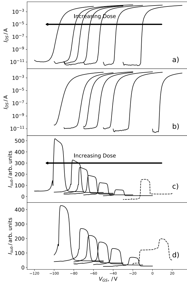
Fig. 6: a) Transfer characteristics of ILDMOS type I and b) of ILDMOS type II with V_{DS} = 3.3 V for increasing irradiation dose. Corresponding gated-diode substrate current measurements are shown in c) and d) for ILDMOS type I and II, respectively.
