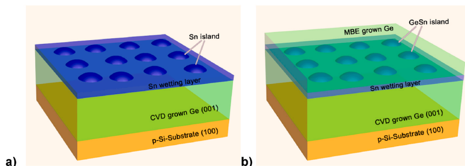
Fig. 1. (a) Schematic view of uncapped Sn-rich islands grown on a Ge/Si (100) substrate by molecular beam epitaxy (b) Schematic view of the Ge-capped Sn islands.
