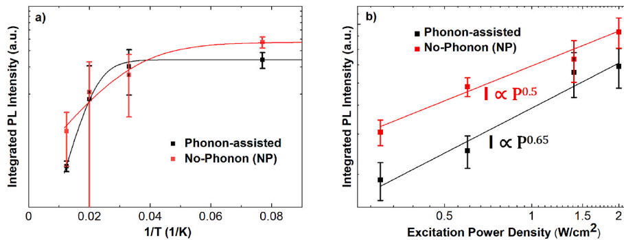
Fig. 5. a) Semi-logarithmic plot of the integrated PL intensities of the phonon-assisted and NP peaks as a function of inverse lattice temperature together with results from Arrhenius fits. b) A power-law relation can be found between the integrated PL intensities and the excitation power density whose exponent points towards Auger recombination as the dominant non-radiative recombination channel.
