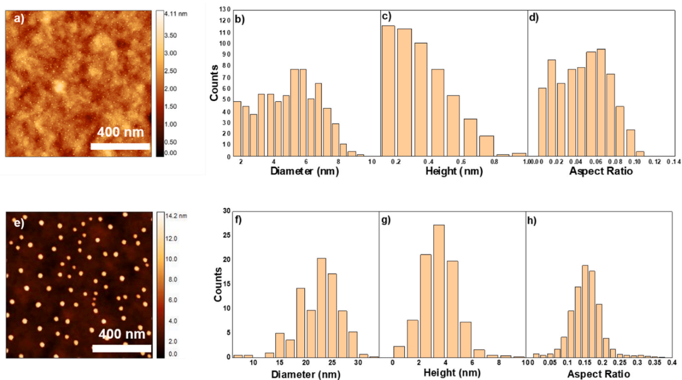
Fig. 2. a) AFM image ( 1 \times 1 \mu\text{m}^2 ) of Sample A at the onset of Sn-rich island formation as can be seen from the histograms of b) diameters, c) heights and d) aspect ratios of the dots. The 1 \times 1 \mu\text{m}^2 AFM image e) of Sample B shows the presence of much larger dots, with histograms of f) diameters, g) heights and h) aspect ratios that have Gaussian shapes.
