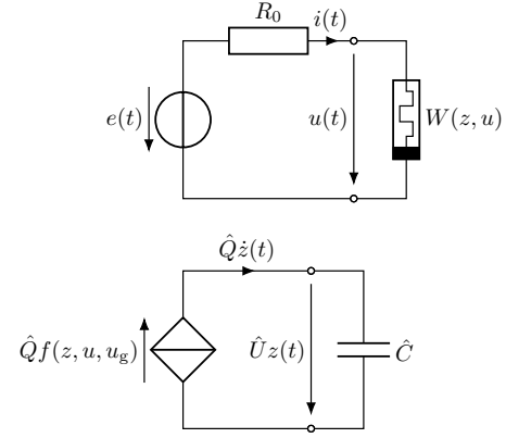
Fig. 2: Emulation scenario, where the bottom circuit represents a circuit-theoretical method of calculating the internal state. The constants \hat{C} = 1 F and \hat{Q} = 1 C are normalization constants with the unit of capacitance and charge, respectively.
