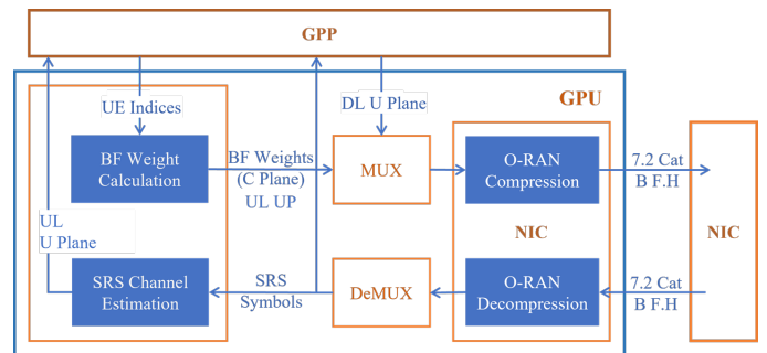
Figure III-1 GPU-based offloading engine
