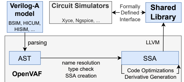
Figure 3: Overview of the OpenVAF Verilog-A compiler
