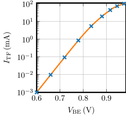
Figure 4: Example: Transfer current of HICUM/L2 from the Verilog-AE Python backend of OpenVAF [24].
