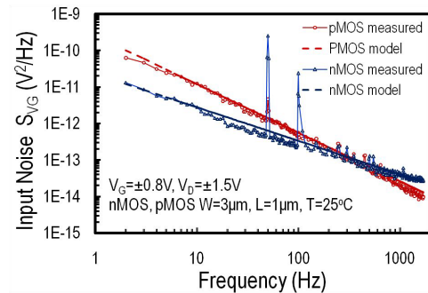
Figure 1: Comparison of EKV 2.6 simu/meas data of the input power spectral density S_{VG}(f) for 180nm CMOS process.
