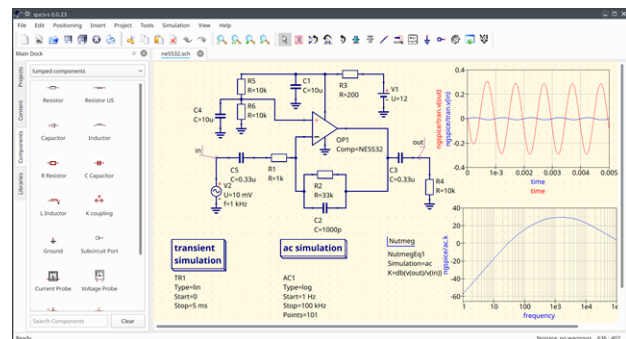
Figure 2: Qucs-S simulation example with backend ngspice.
