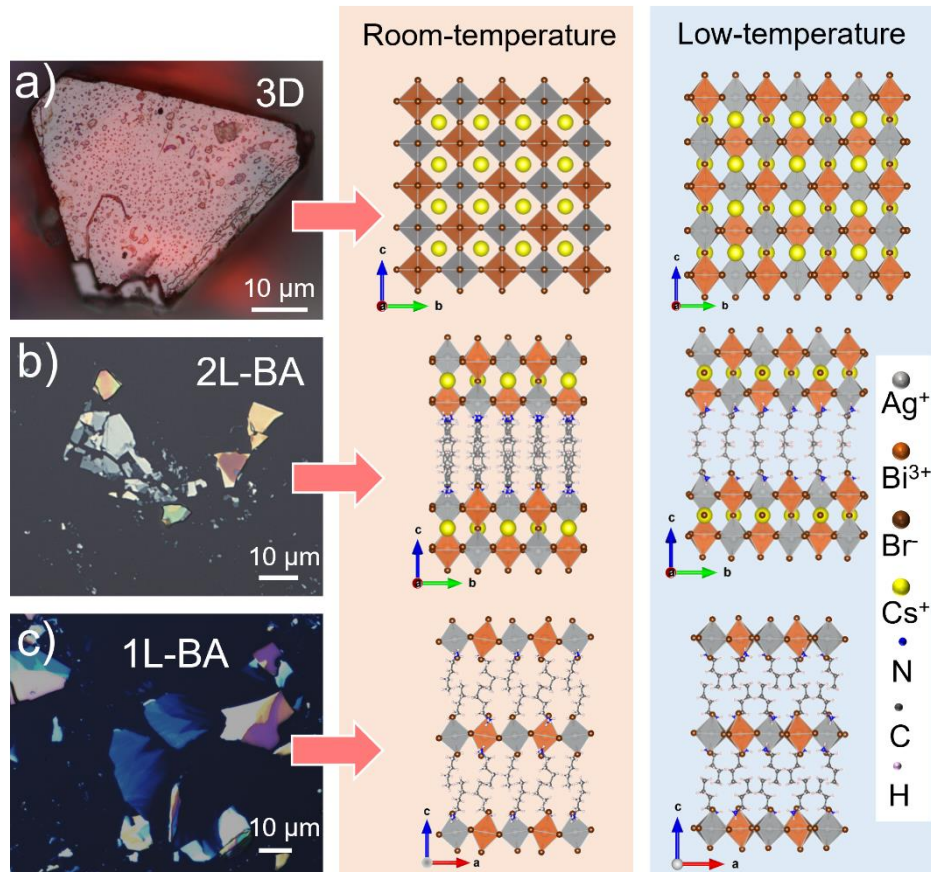
Figure 1. Optical microscope images of the different double perovskite structures: (a) 3D \text{Cs}_2\text{AgBiBr}_6 microcrystals and mechanically exfoliated 2L-BA (b) and 1L-BA (c) flakes on \text{SiO}_2/\text{Si} substrates together with their crystal structures drawn using VESTA 3 software [44] based on the crystallographic data from refs. [15,26] .
