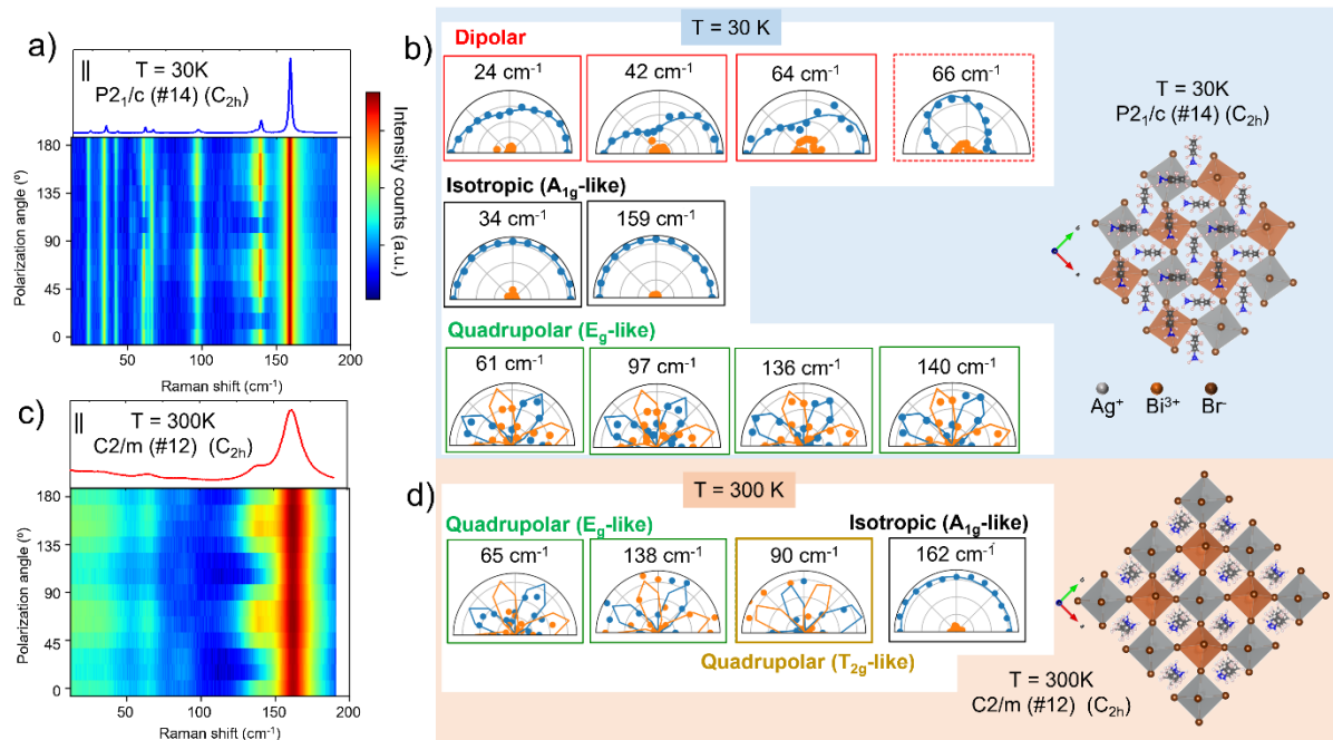
Figure 6. Angle dependence of the phonon modes of the 1L-BA sample: (a, c) Color plots of polarized-dependent Raman spectra at 30K and 300K, respectively, (see Figure S6 in the SI for angle dependent Raman spectra in depolarized configuration). (b) Polar plots of the Raman mode intensities (dots) extracted from the data in Figure 6a,b and Figure S6, and best fits (lines) obtained from the corresponding Raman tensor equations. Polarized data is shown in blue, depolarized in orange. The top view on the crystal structure of the 1L sample at 30K and 300K using VESTA software [44] is also displayed. The orientation of the principal axes in the octahedra plane is the same as for the polar plots.
