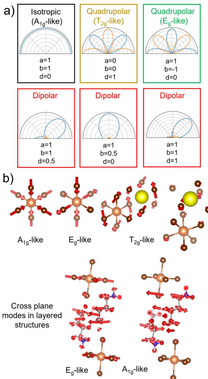
Figure 4. (a) Polar plots of the Raman mode calculated from the Raman tensor for selected values for its components. (b) Vibrational motions of the different modes obtained by DFT
