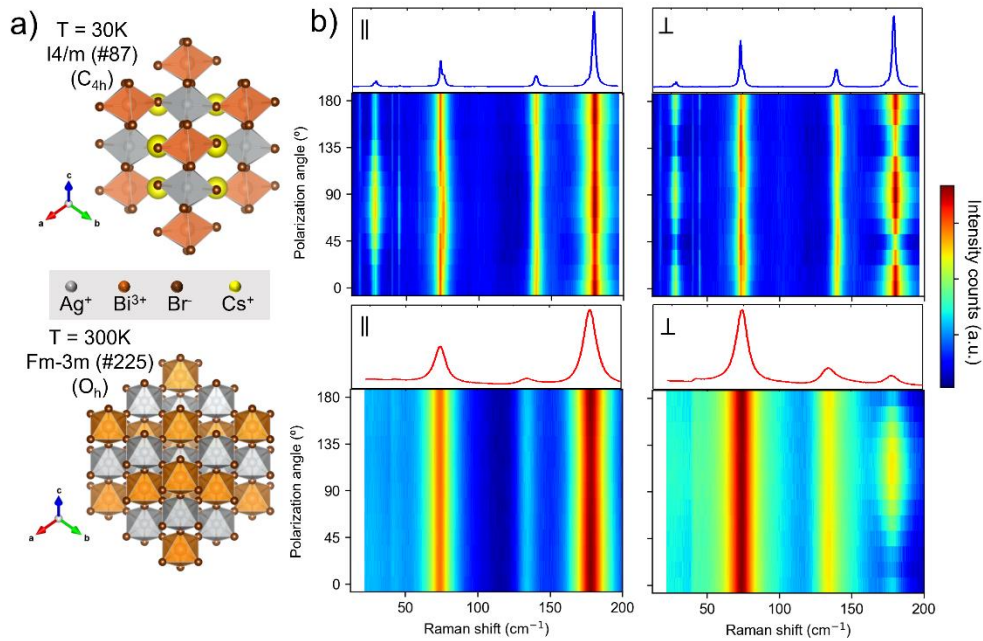
Figure 3. (a) Crystal structures of the 3D \text{Cs}_2\text{AgBiBr}_6 PSK drawn using VESTA software [44] for the low- and high-temperature phases [26] from the perspective of the (111) plane that is exposed in the experiment. (b) Color plots of the angle dependence of the Raman spectrum for polarized ( \parallel ) and depolarized ( \perp ) configurations. The integrated Raman spectra along the polarization angle are shown on top of the color plots.
