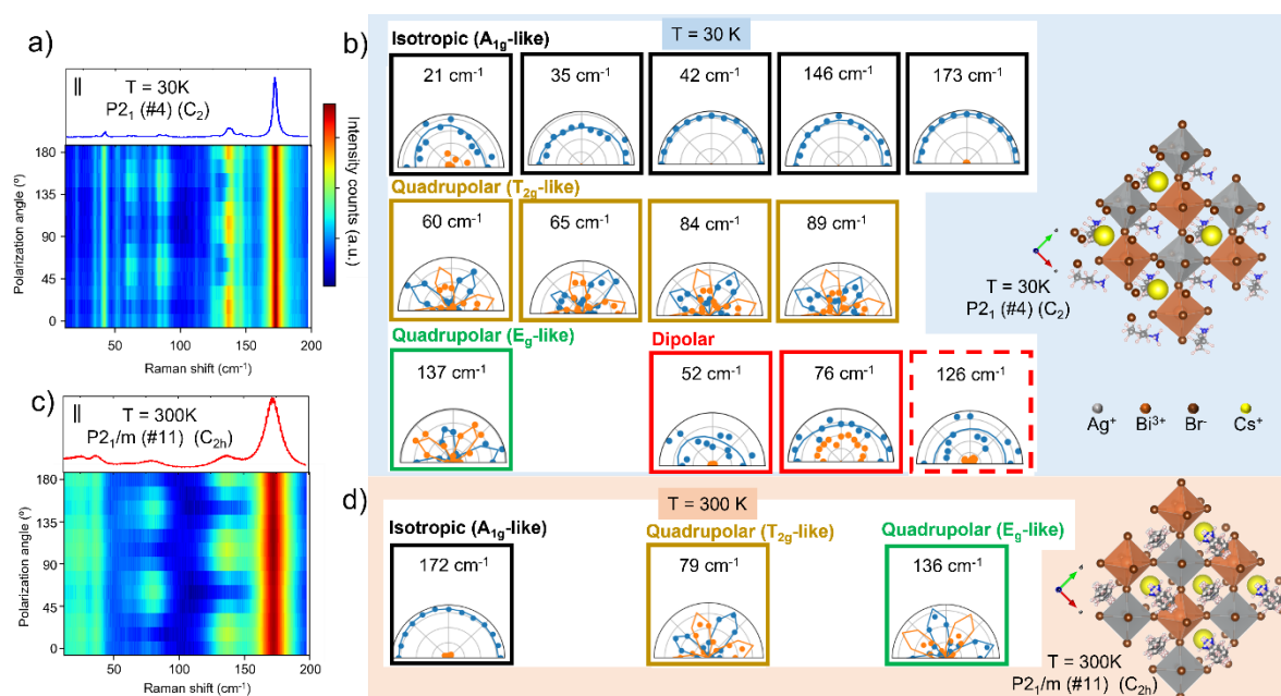
Figure 5. Angle dependence of the phonon modes of the 2L-BA sample: (a, c) Color plots of the polarized angle-dependent Raman spectra recorded at 30K and 300K, respectively (see Figure S5 in the SI for angle dependent Raman spectra in depolarized configuration). (b, d) Polar plots of the Raman mode intensities (dots) extracted from the data in Figure 5a,b and Figure S5, and best fits (lines) obtained from the corresponding Raman tensor equations. Polarized data is shown in blue, depolarized in orange. The top view on the crystal structure of the 2L sample at 30K and 300K using VESTA software [44] is also shown. The orientation of the principal axes in the octahedra plane is the same as in the polar plots.
